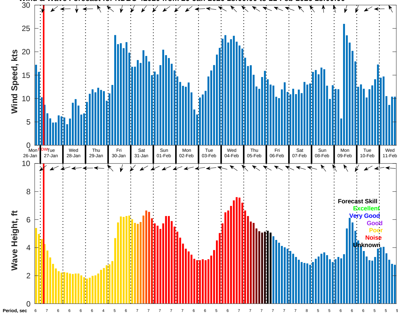
Wind & Wave Forecast for NDBC 42020 from 26-Jan-2026 18:00:00 to 11-Feb-2026 18:00:00
