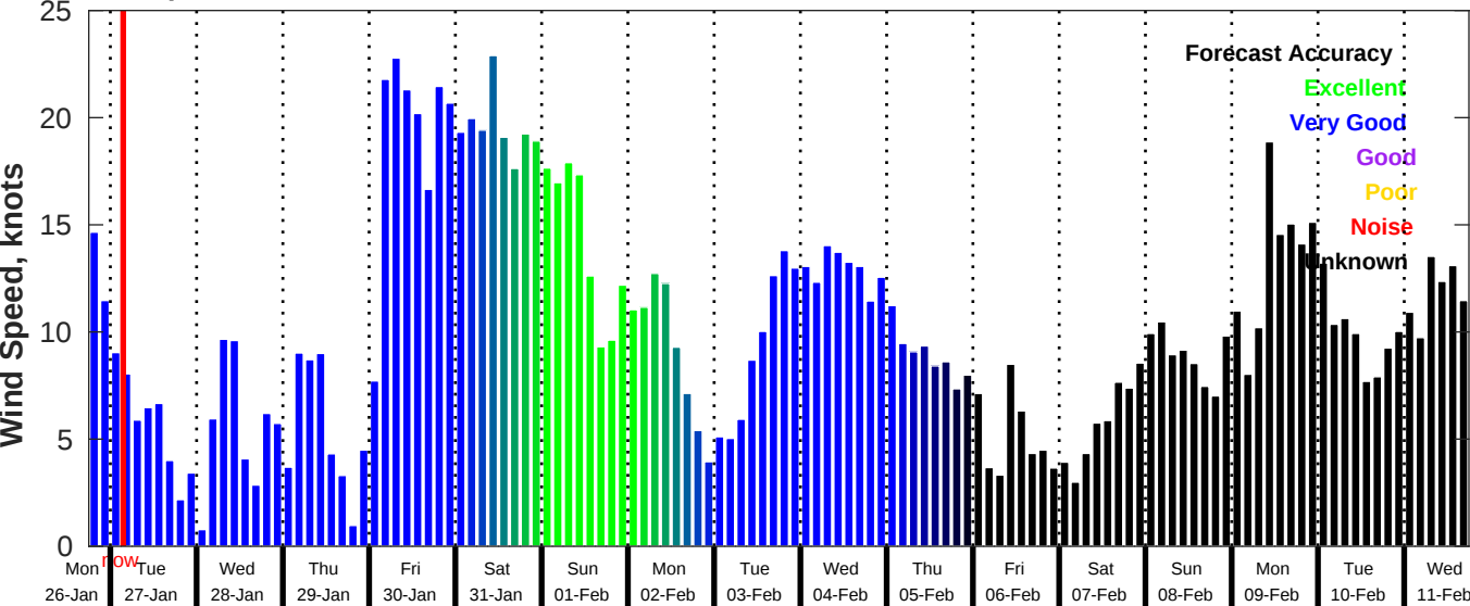
GFS Wind Speed Forecast for NDBC 42035 from 26-Jan-2026 18:00:00 to 11-Feb-2026 18:00:00
