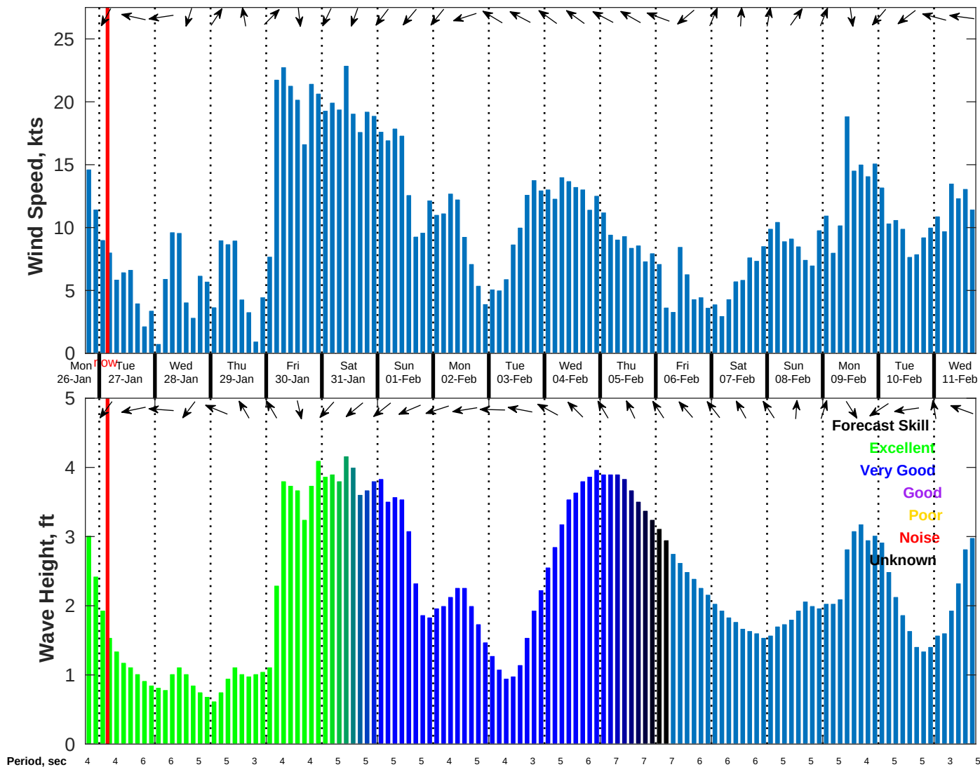
Wind & Wave Forecast for NDBC 42035 from 26-Jan-2026 18:00:00 to 11-Feb-2026 18:00:00
