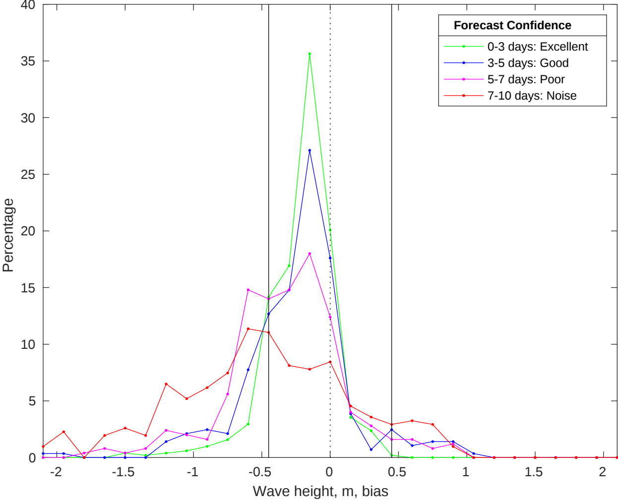
NDBC 42036 vs CMEMS Waves Bias Histogram: 27-Jan-2026
