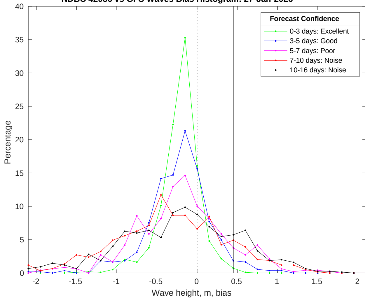
NDBC 42036 vs GFS Waves Bias Histogram: 27-Jan-2026
