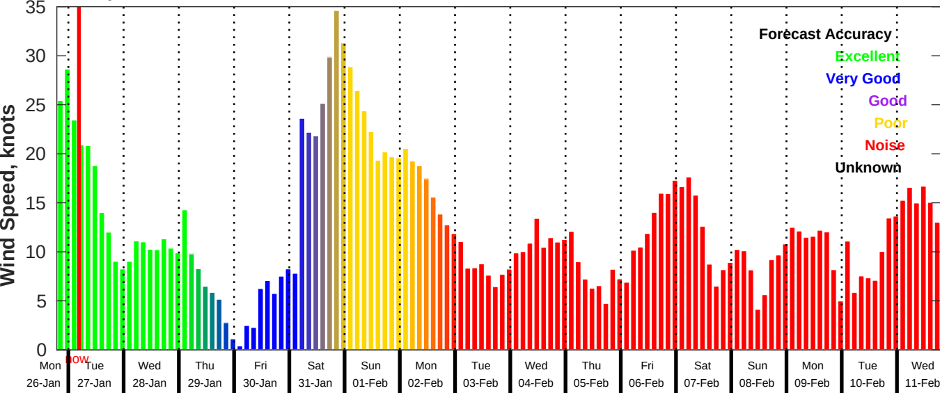
GFS Wind Speed Forecast for NDBC 42036 from 26-Jan-2026 19:00:00 to 11-Feb-2026 19:00:00
