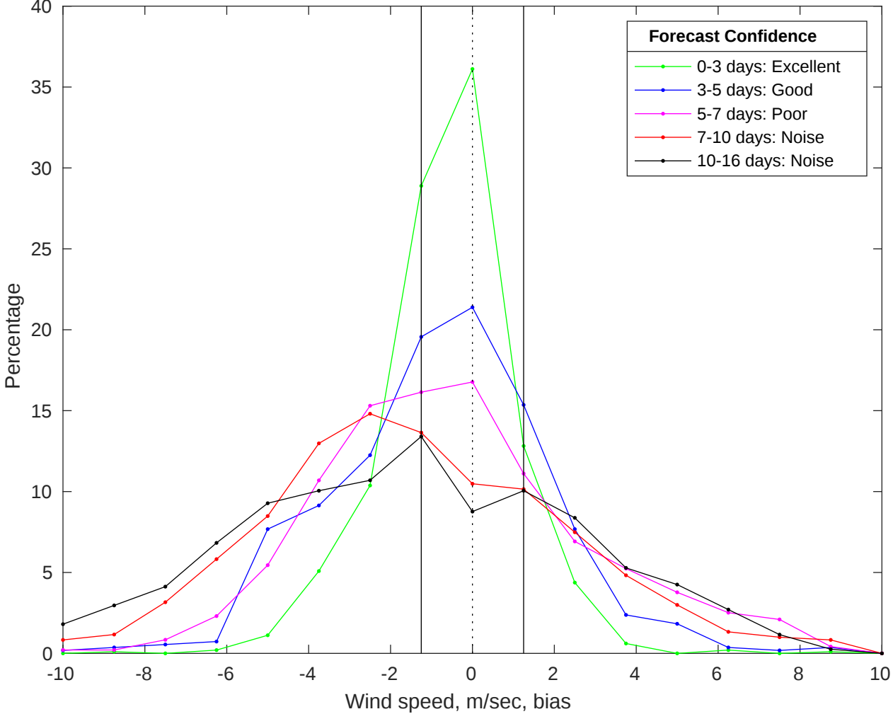
NDBC 42040 vs GFS Winds Bias Histogram: 27-Jan-2026
