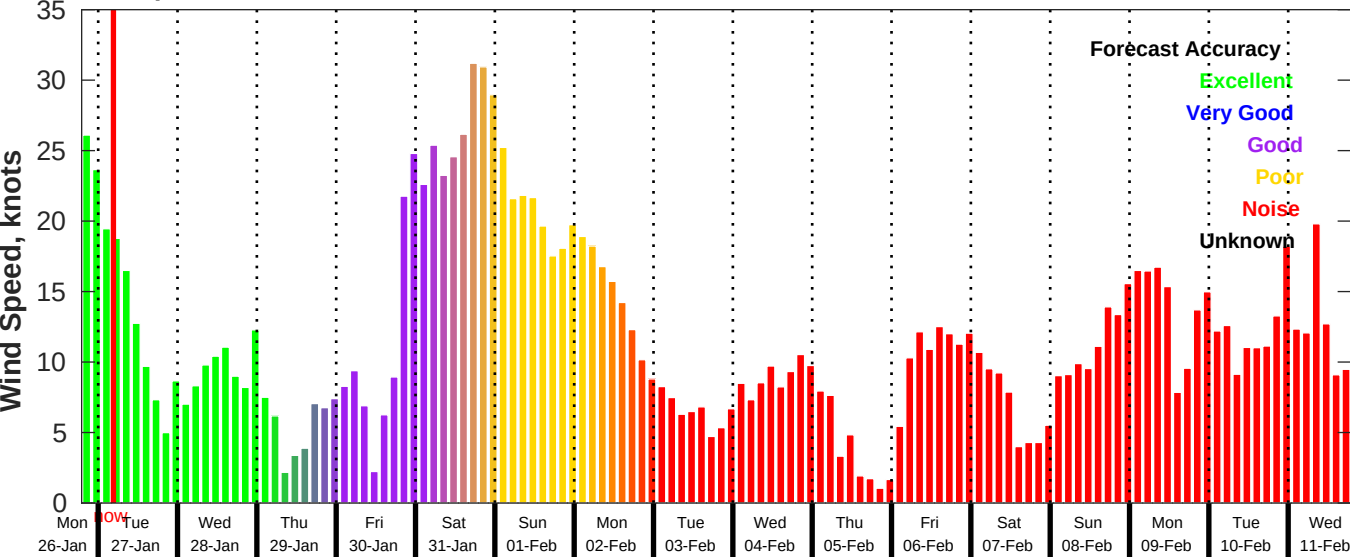
GFS Wind Speed Forecast for NDBC 42040 from 26-Jan-2026 19:00:00 to 11-Feb-2026 19:00:00
