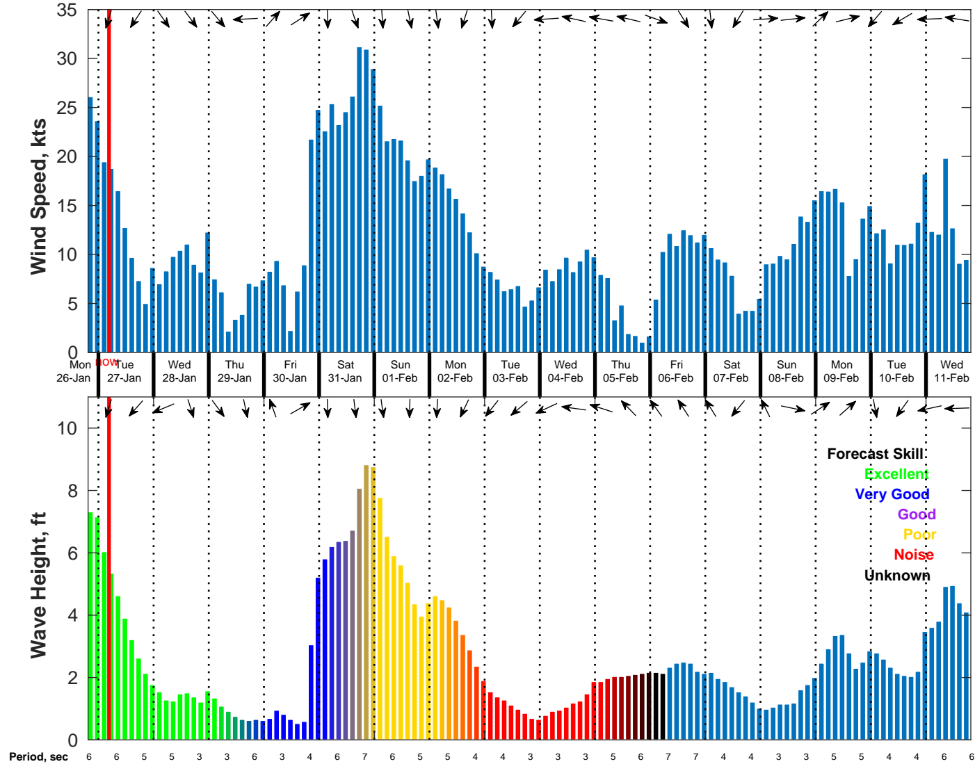
Wind & Wave Forecast for NDBC 42040 from 26-Jan-2026 19:00:00 to 11-Feb-2026 19:00:00
