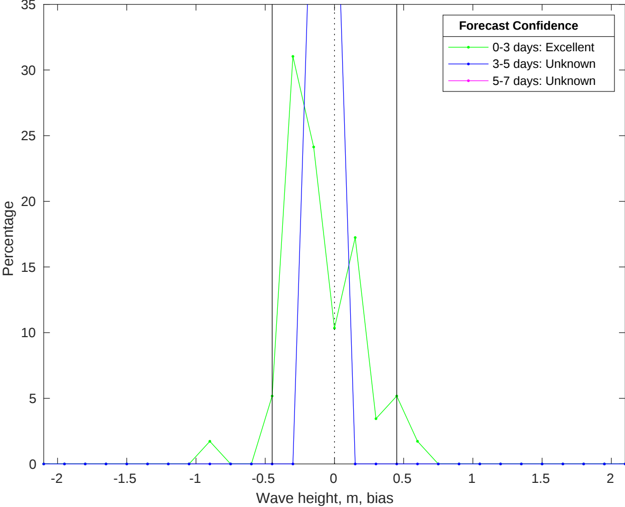
NDBC 42058 vs CMEMS Waves Bias Histogram: 27-Jan-2026
