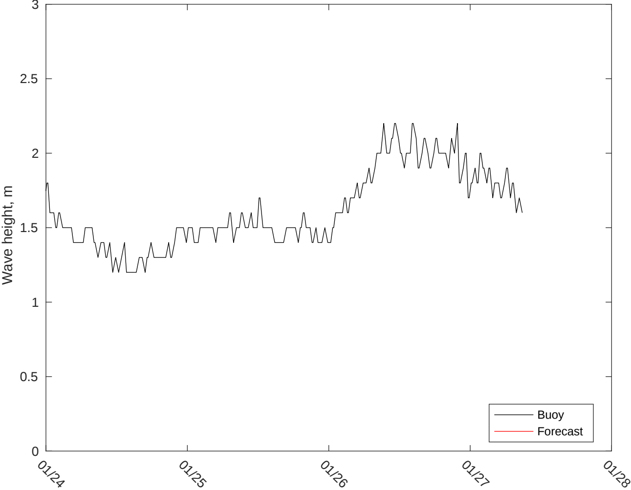
NDBC 42058 vs GFS Waves: 10 to 16 day forecast
