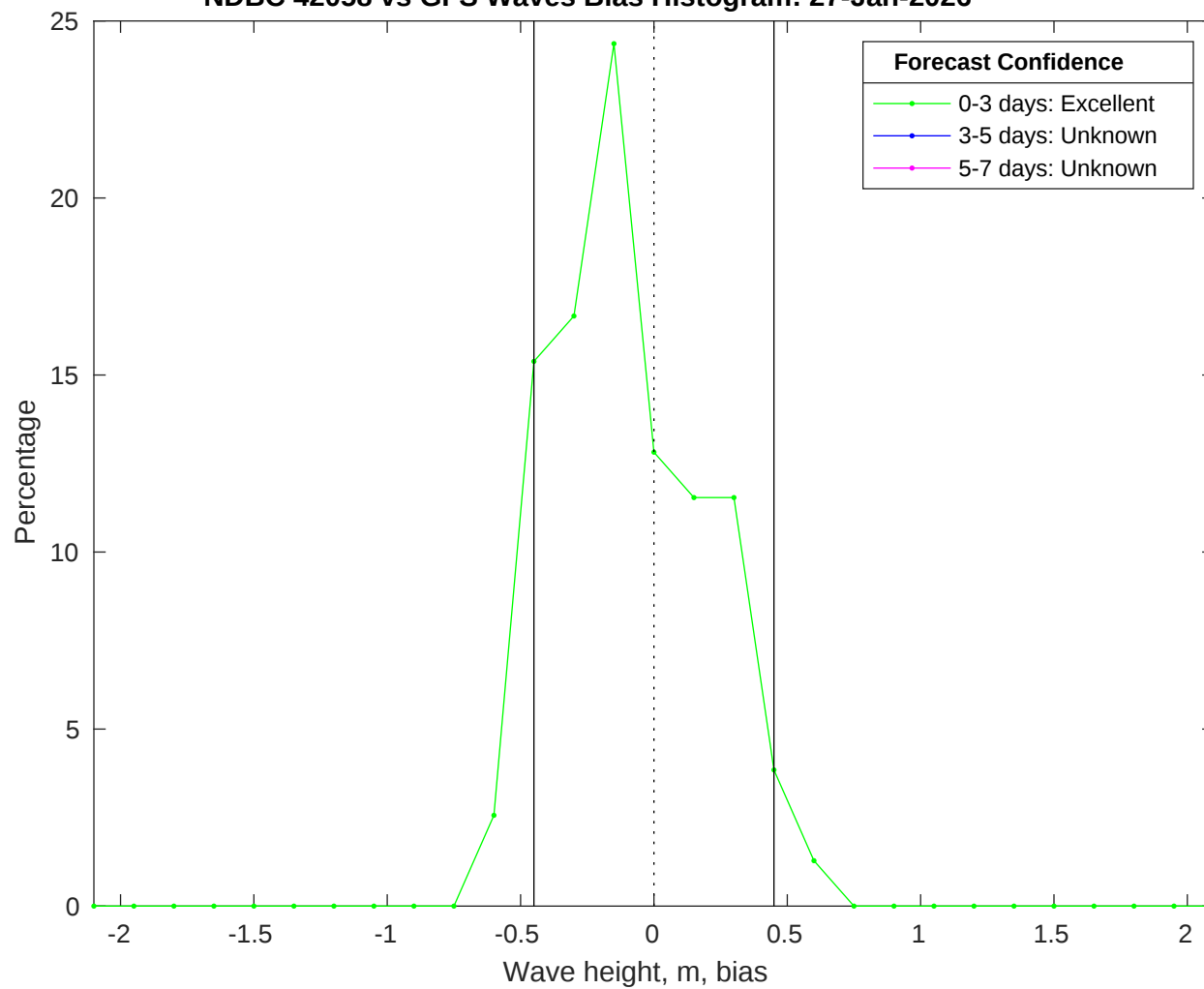
NDBC 42058 vs GFS Waves Bias Histogram: 27-Jan-2026
