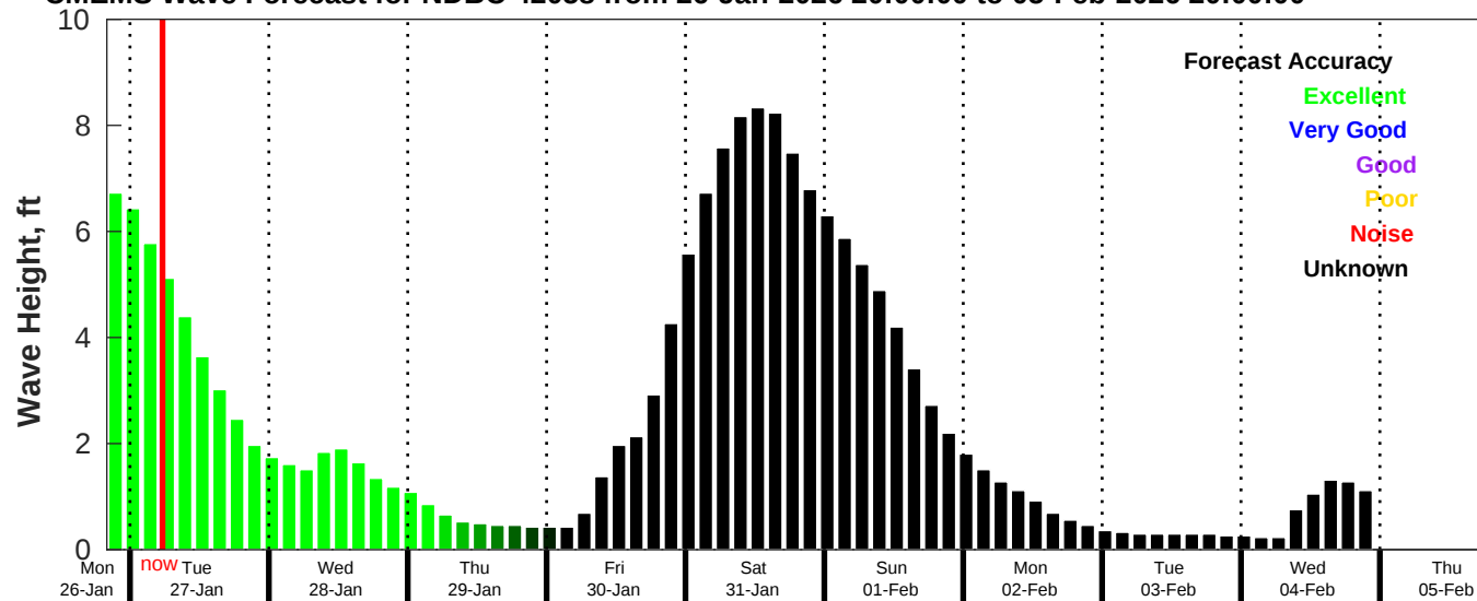
CMEMS Wave Forecast for NDBC 42058 from 26-Jan-2026 20:00:00 to 05-Feb-2026 20:00:00
