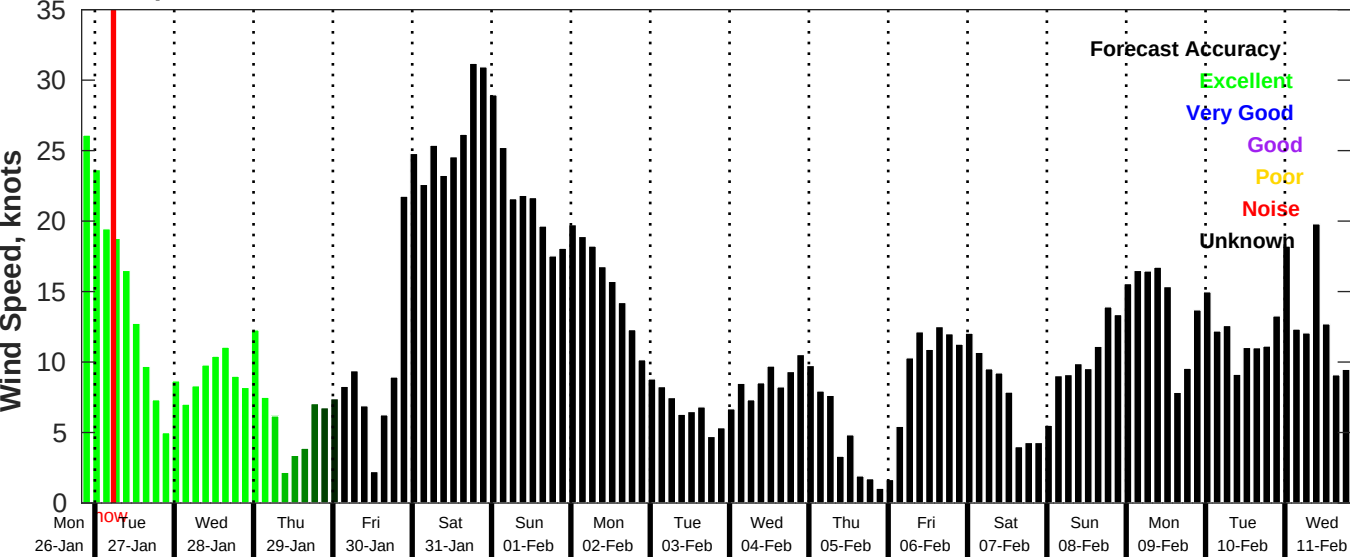
GFS Wind Speed Forecast for NDBC 42058 from 26-Jan-2026 20:00:00 to 11-Feb-2026 20:00:00
