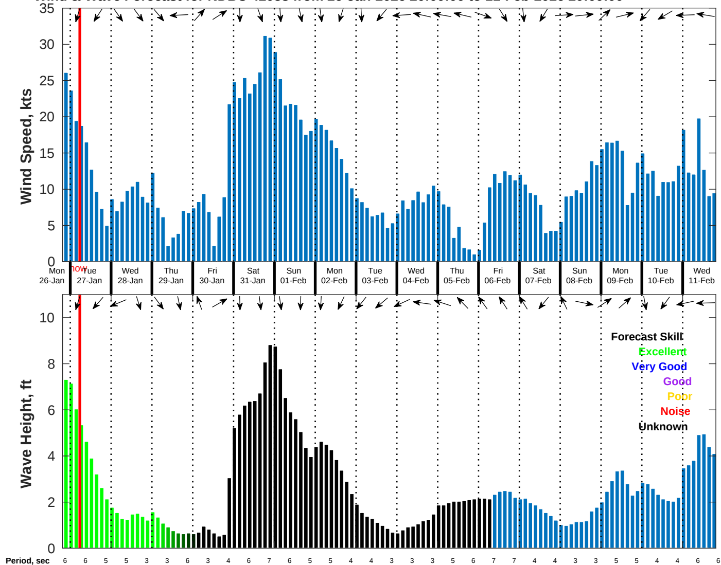
Wind & Wave Forecast for NDBC 42058 from 26-Jan-2026 20:00:00 to 11-Feb-2026 20:00:00
