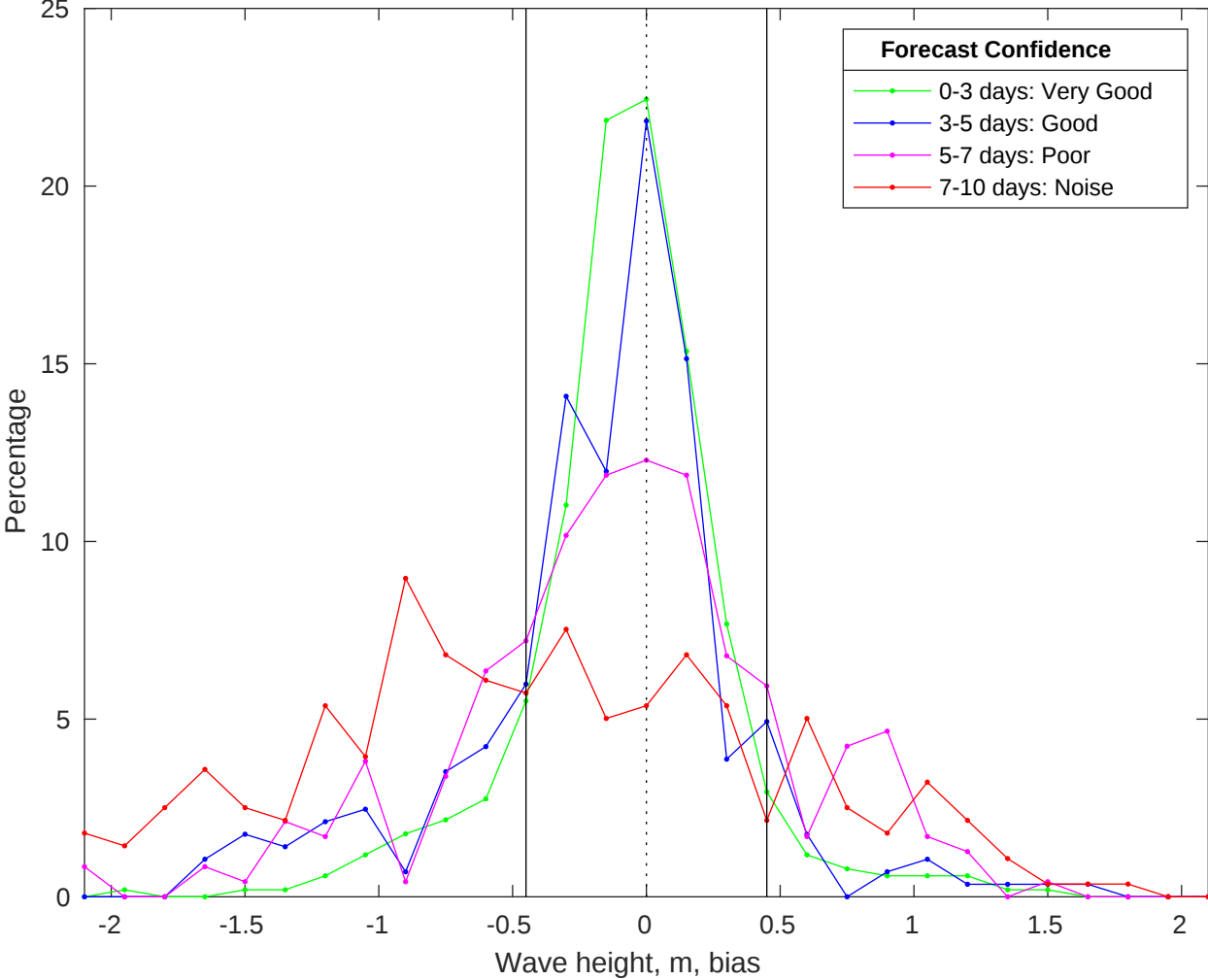
NDBC 44008 vs CMEMS Waves Bias Histogram: 27-Jan-2026
