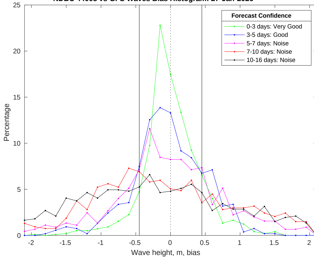
NDBC 44008 vs GFS Waves Bias Histogram: 27-Jan-2026
