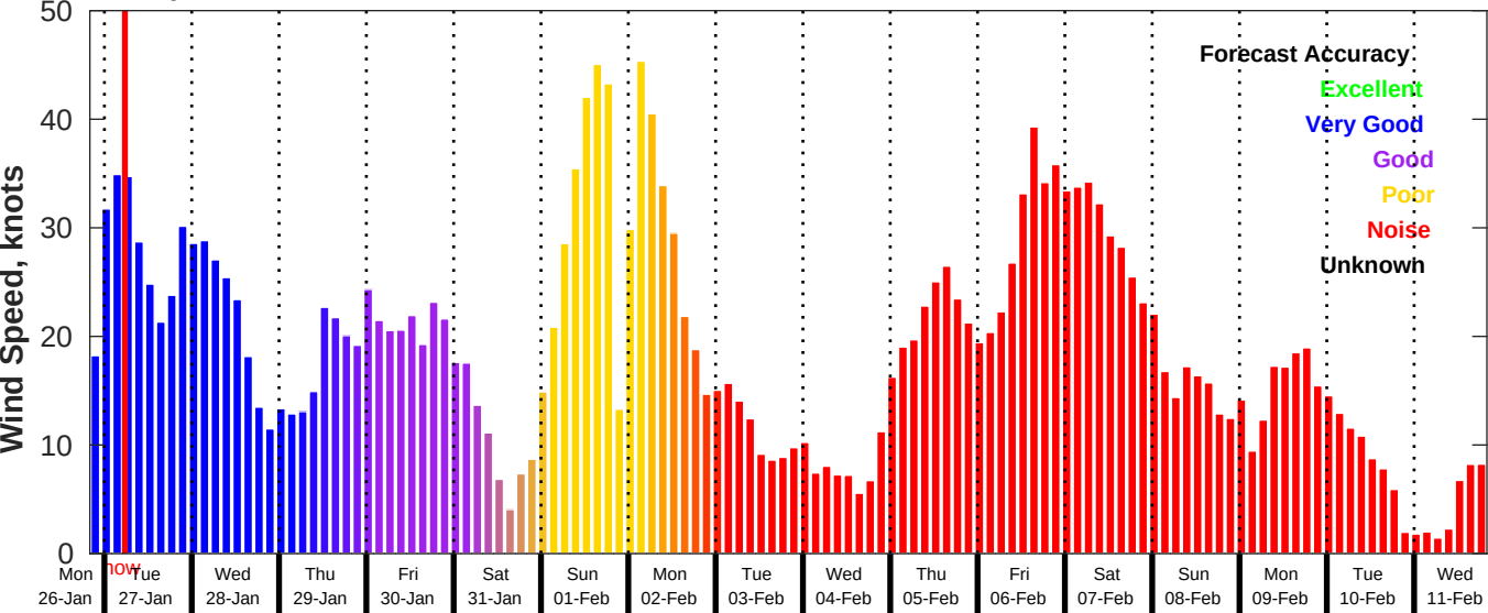
GFS Wind Speed Forecast for NDBC 44008 from 26-Jan-2026 20:00:00 to 11-Feb-2026 20:00:00
