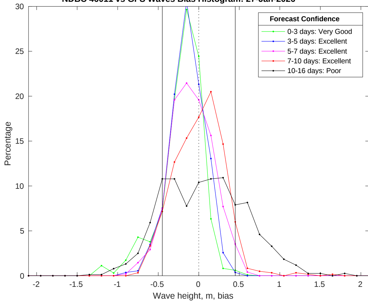
NDBC 46011 vs GFS Waves Bias Histogram: 27-Jan-2026
