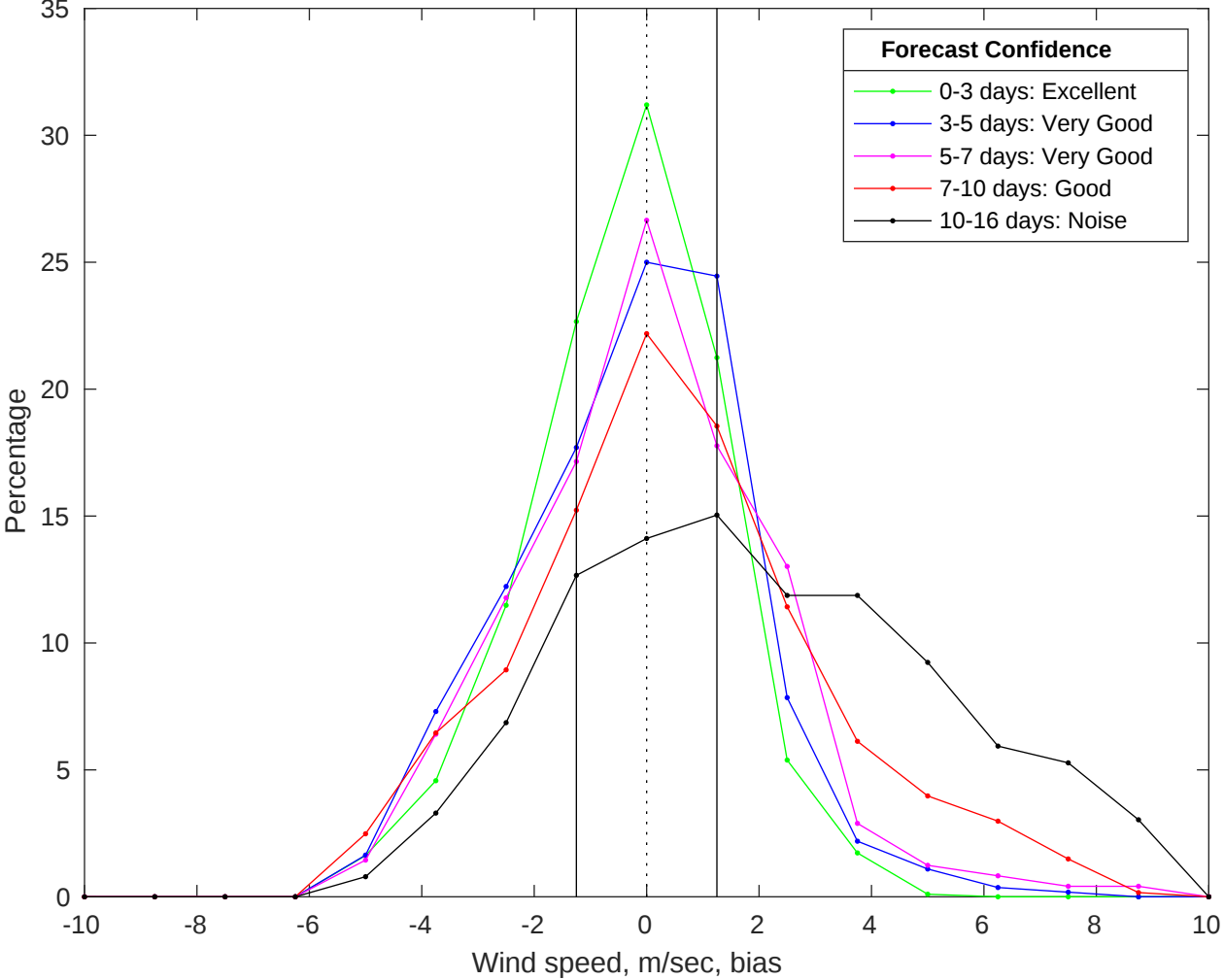
NDBC 46011 vs GFS Winds Bias Histogram: 27-Jan-2026
