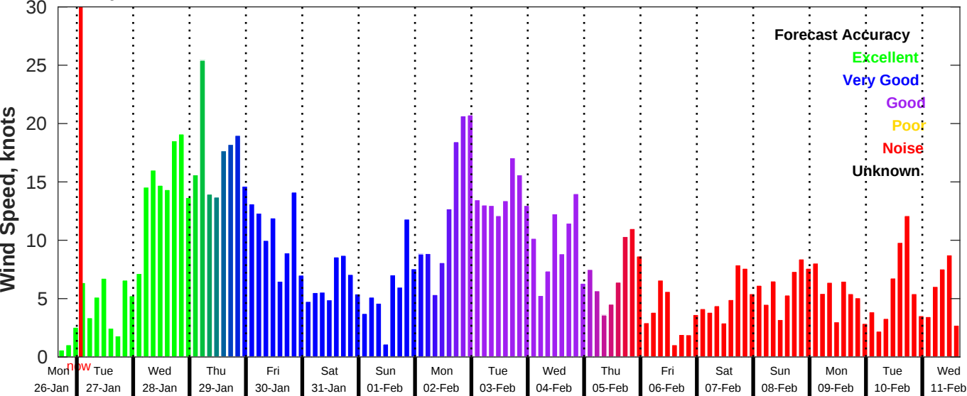
GFS Wind Speed Forecast for NDBC 46011 from 26-Jan-2026 16:00:00 to 11-Feb-2026 16:00:00
