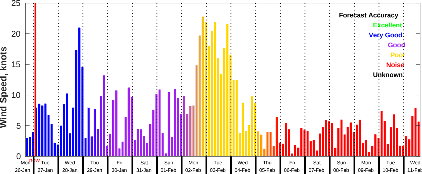
GFS Wind Speed Forecast for NDBC 46028 from 26-Jan-2026 16:00:00 to 11-Feb-2026 16:00:00
