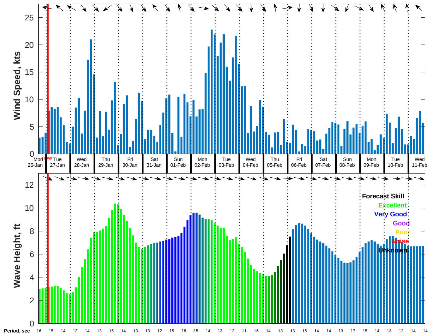
Wind & Wave Forecast for NDBC 46028 from 26-Jan-2026 16:00:00 to 11-Feb-2026 16:00:00
