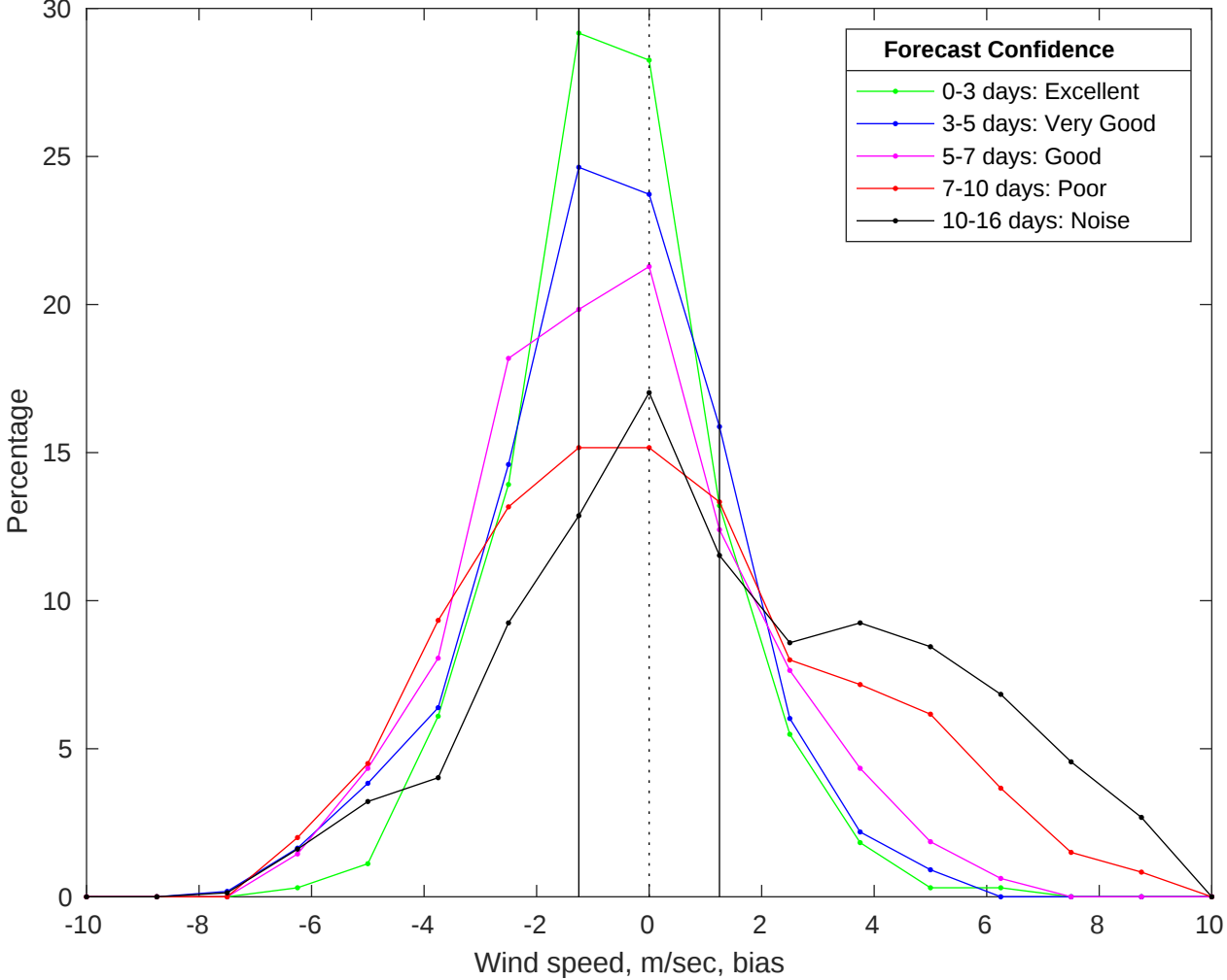
NDBC 46054 vs GFS Winds Bias Histogram: 27-Jan-2026
