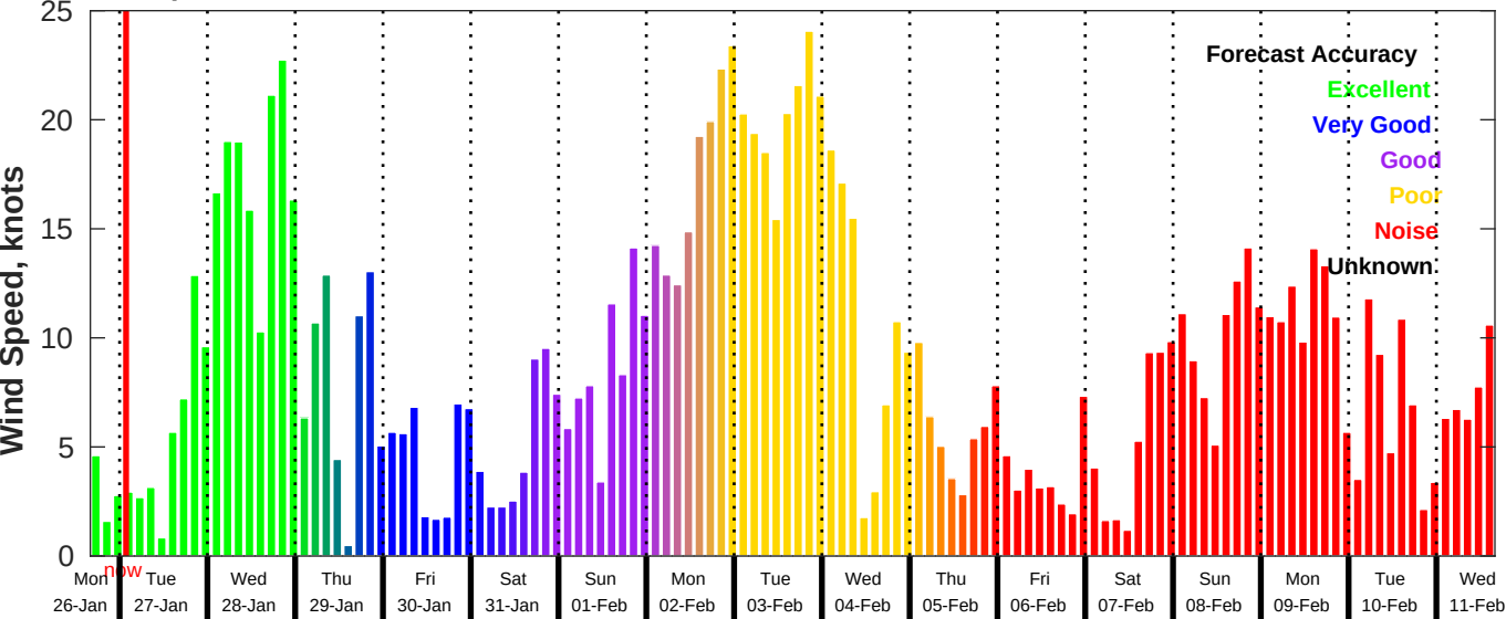
GFS Wind Speed Forecast for NDBC 46054 from 26-Jan-2026 16:00:00 to 11-Feb-2026 16:00:00
