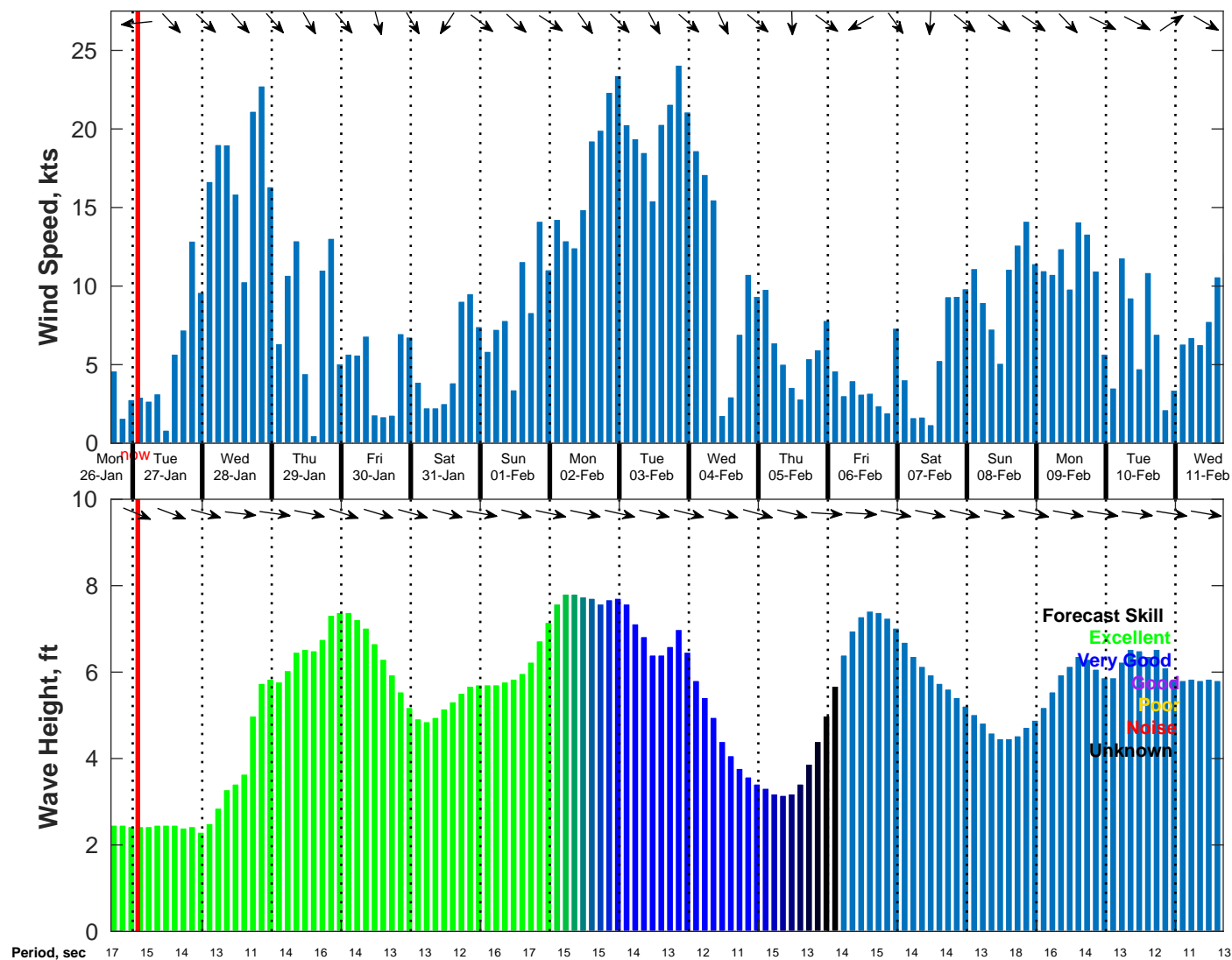
Wind & Wave Forecast for NDBC 46054 from 26-Jan-2026 16:00:00 to 11-Feb-2026 16:00:00
