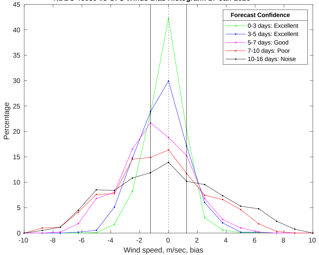
NDBC 46059 vs GFS Winds Bias Histogram: 27-Jan-2026
