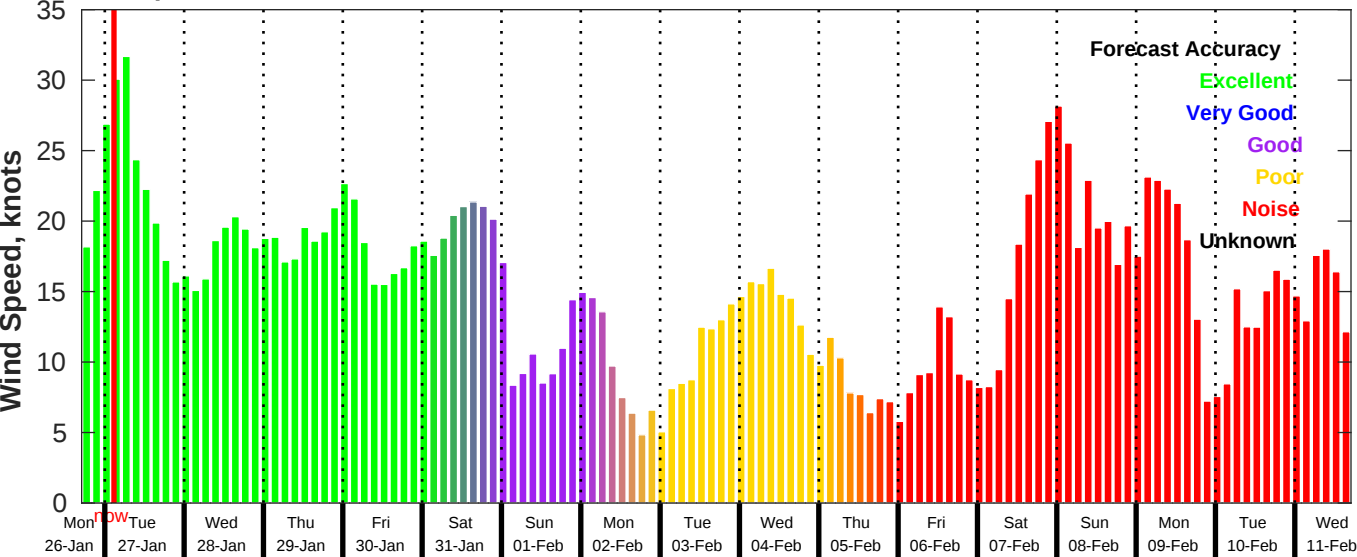
GFS Wind Speed Forecast for NDBC 46059 from 26-Jan-2026 17:00:00 to 11-Feb-2026 17:00:00
