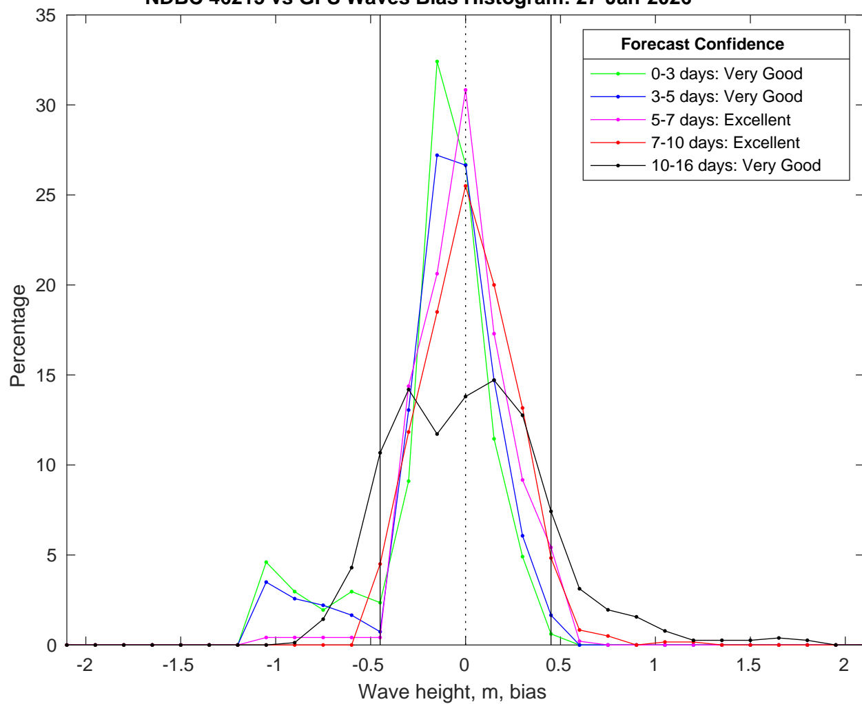
NDBC 46215 vs GFS Waves Bias Histogram: 27-Jan-2026
