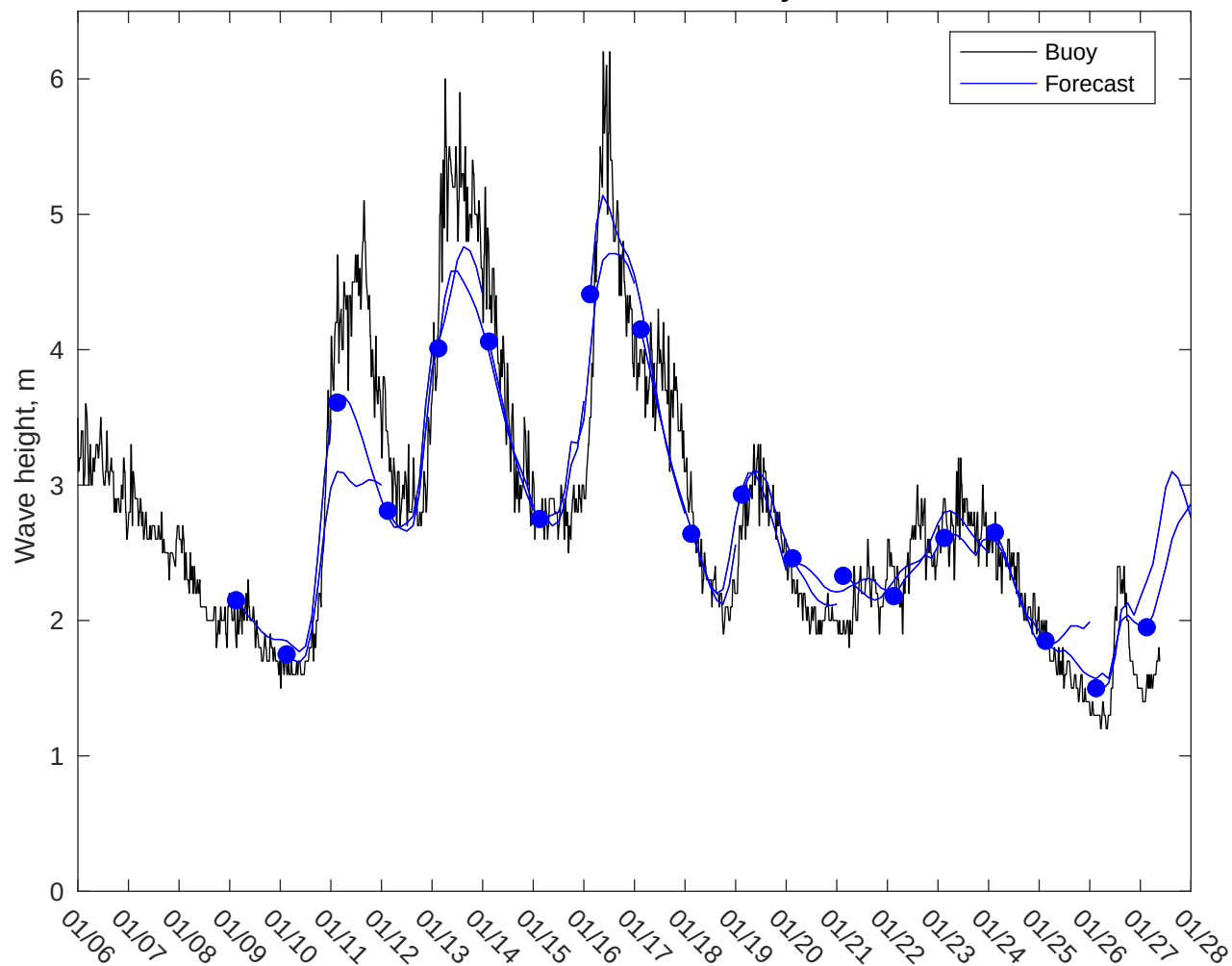
NDBC 51000 vs CMEMS Waves: 3 to 5 day forecast
