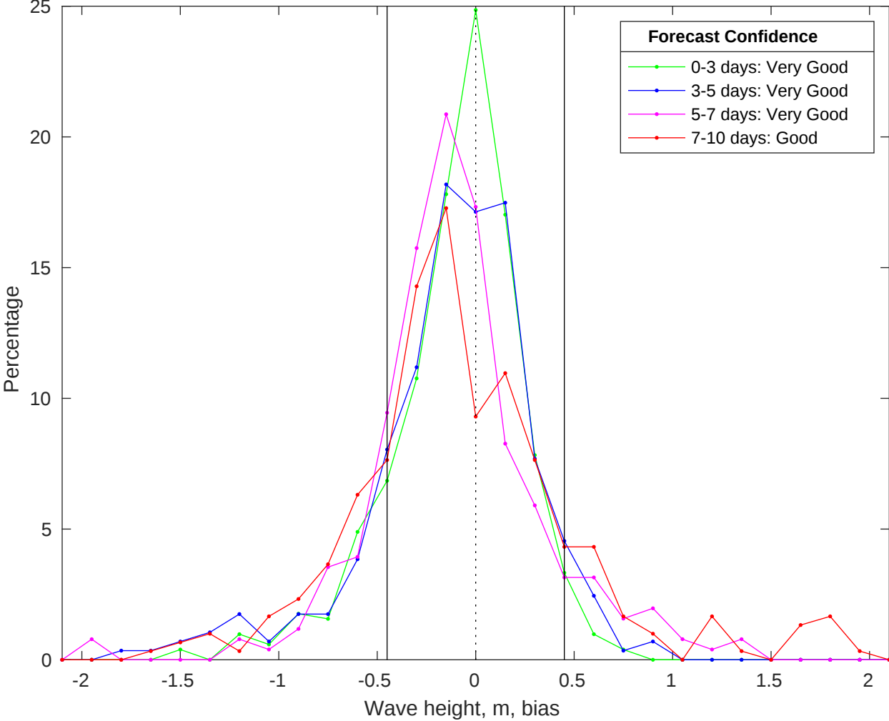
NDBC 51000 vs CMEMS Waves Bias Histogram: 27-Jan-2026
