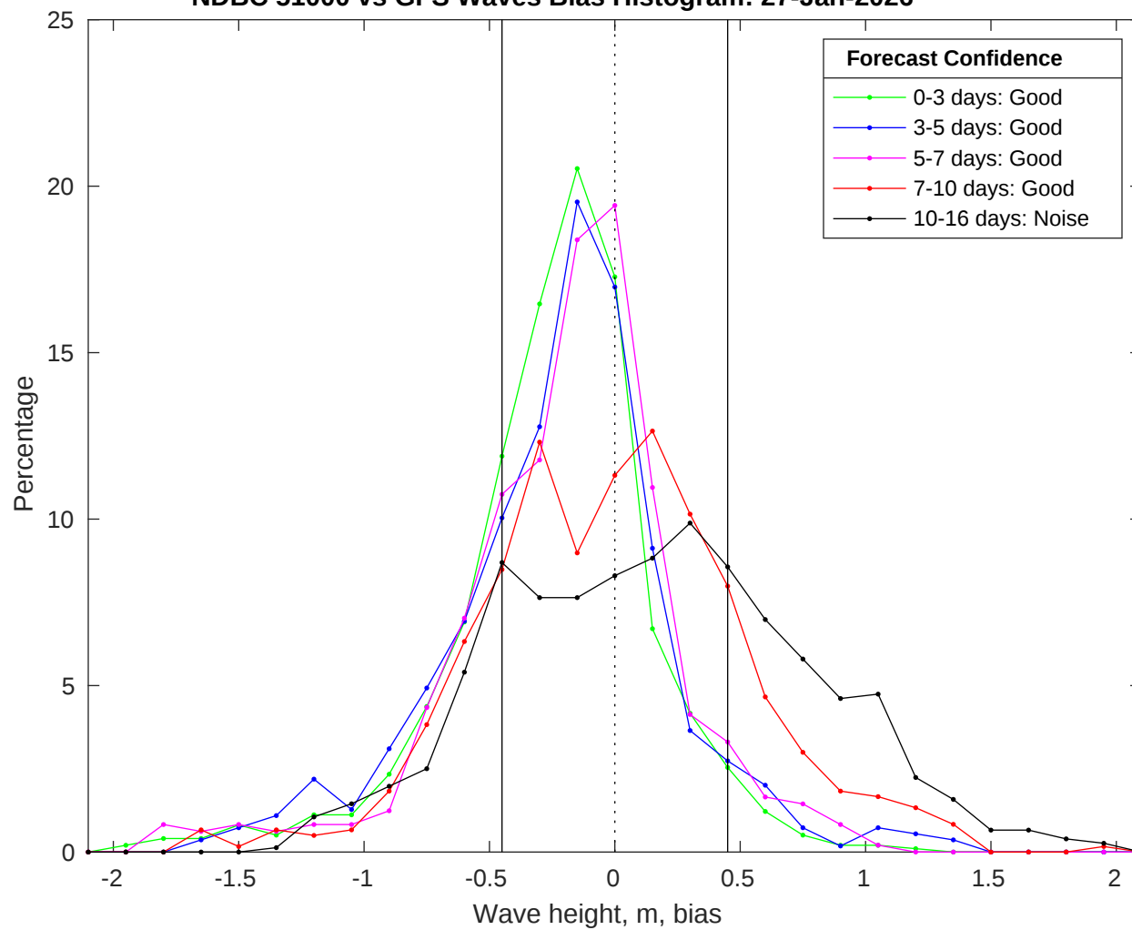
NDBC 51000 vs GFS Waves Bias Histogram: 27-Jan-2026
