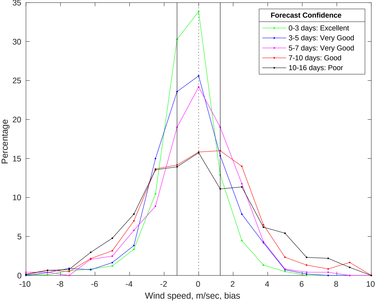
NDBC 51000 vs GFS Winds Bias Histogram: 27-Jan-2026
