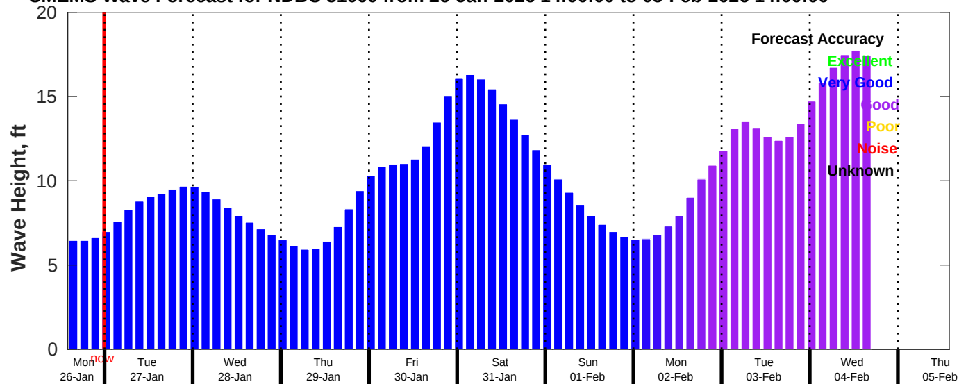
CMEMS Wave Forecast for NDBC 51000 from 26-Jan-2026 14:00:00 to 05-Feb-2026 14:00:00
