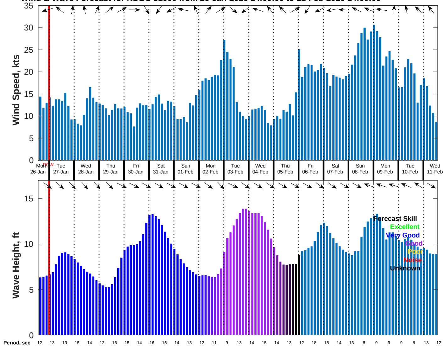
Wind & Wave Forecast for NDBC 51000 from 26-Jan-2026 14:00:00 to 11-Feb-2026 14:00:00
