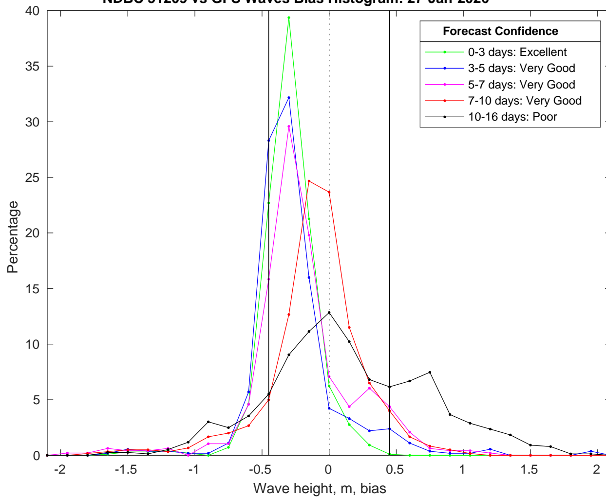
NDBC 51209 vs GFS Waves Bias Histogram: 27-Jan-2026
