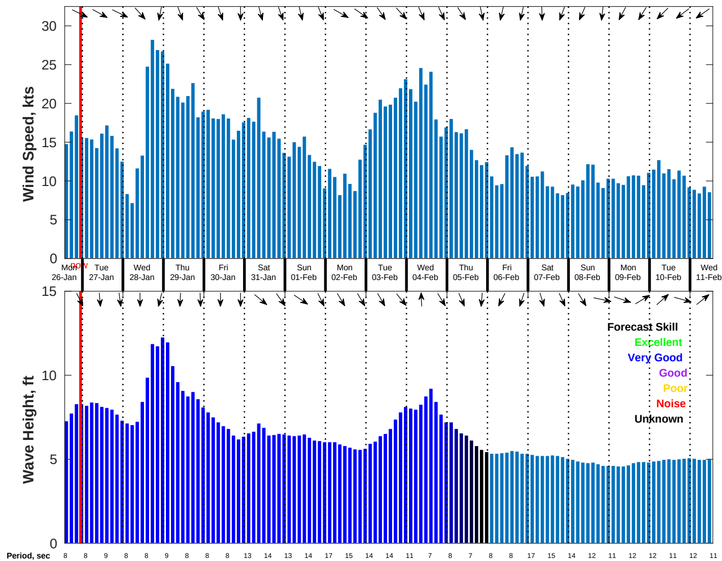
Wind & Wave Forecast for NDBC 51209 from 26-Jan-2026 13:00:00 to 11-Feb-2026 13:00:00
