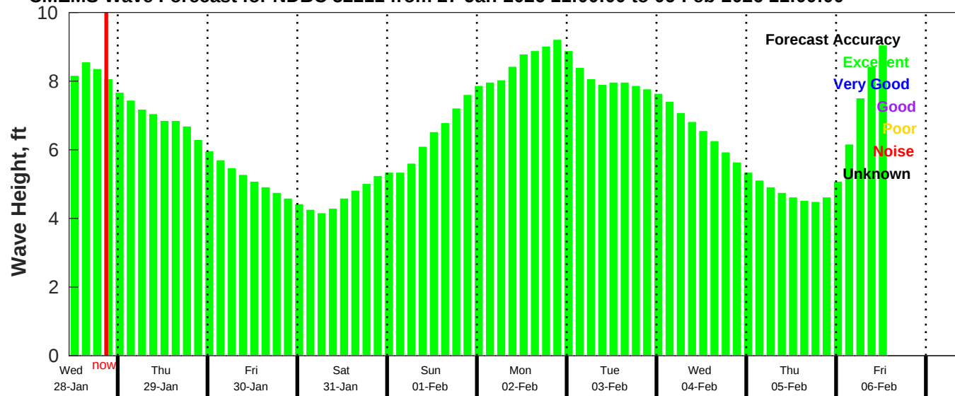
CMEMS Wave Forecast for NDBC 52211 from 27-Jan-2026 11:00:00 to 06-Feb-2026 11:00:00
