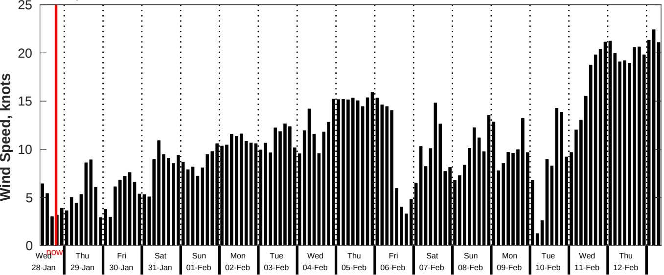
GFS Wind Speed Forecast for NDBC 52212 from 27-Jan-2026 09:00:00 to 12-Feb-2026 09:00:00
