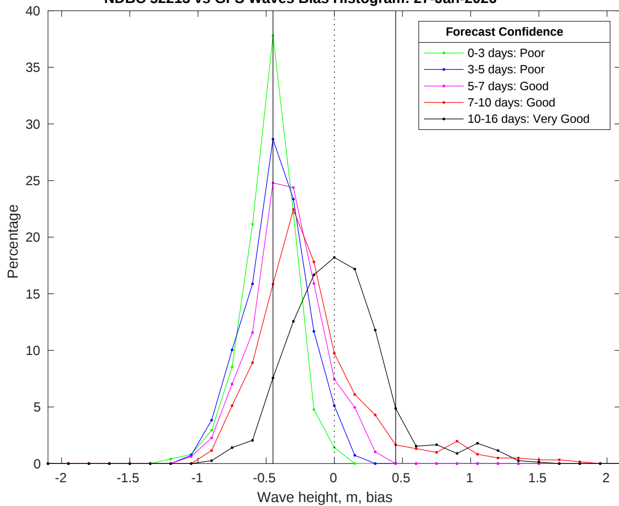
NDBC 52213 vs GFS Waves Bias Histogram: 27-Jan-2026
