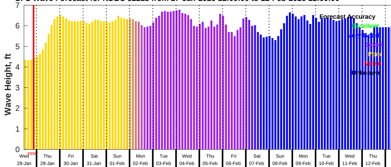
GFS Wave Forecast for NDBC 52213 from 27-Jan-2026 11:00:00 to 12-Feb-2026 11:00:00
