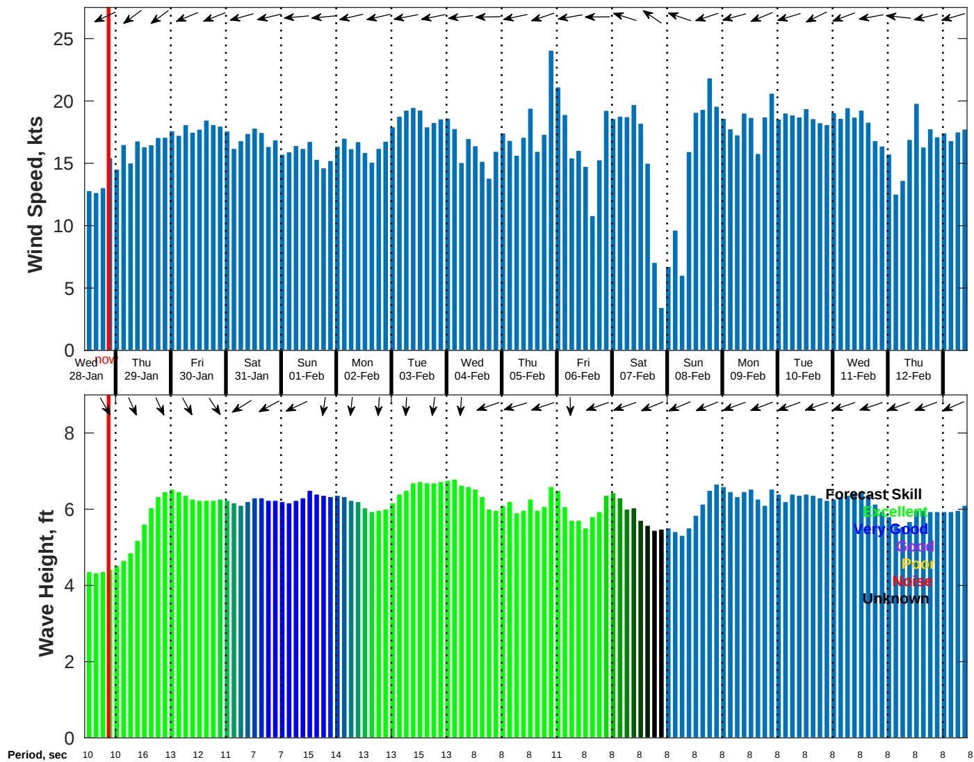
Wind & Wave Forecast for NDBC 52213 from 27-Jan-2026 11:00:00 to 12-Feb-2026 11:00:00
