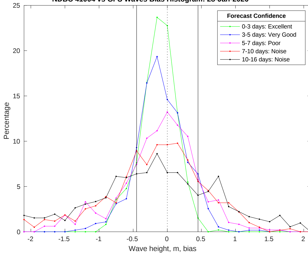
NDBC 41004 vs GFS Waves Bias Histogram: 28-Jan-2026
