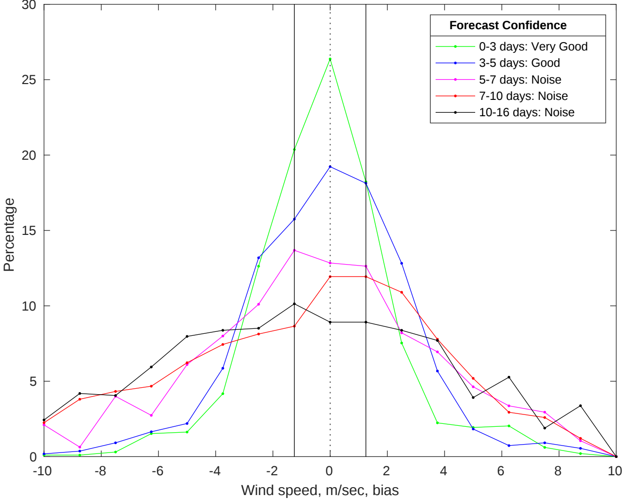
NDBC 41004 vs GFS Winds Bias Histogram: 28-Jan-2026
