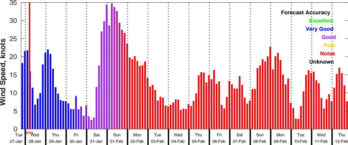
GFS Wind Speed Forecast for NDBC 41004 from 27-Jan-2026 19:00:00 to 12-Feb-2026 19:00:00
