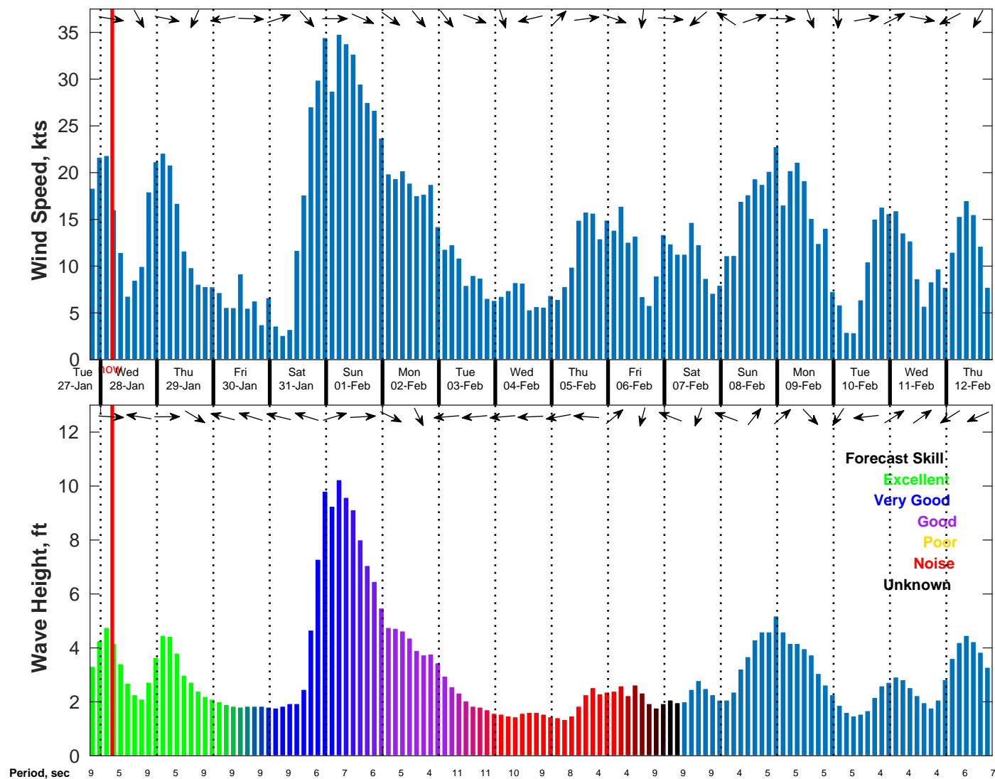
Wind & Wave Forecast for NDBC 41004 from 27-Jan-2026 19:00:00 to 12-Feb-2026 19:00:00
