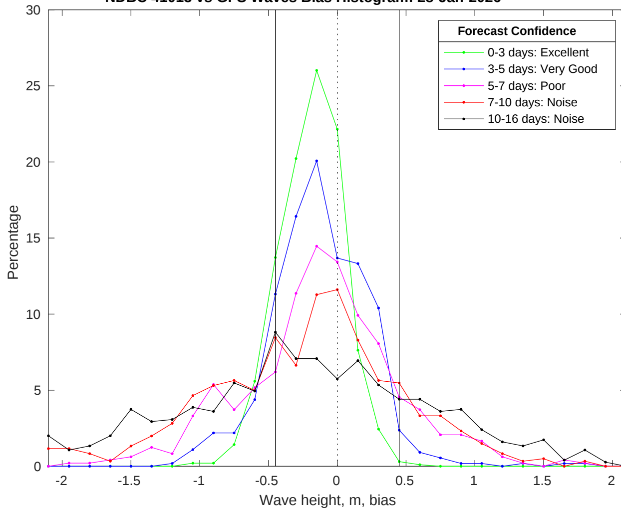
NDBC 41013 vs GFS Waves Bias Histogram: 28-Jan-2026
