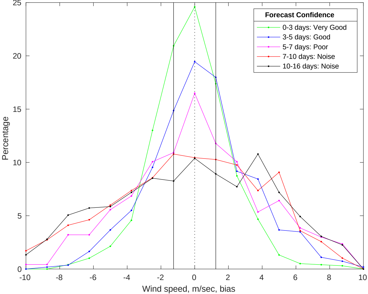
NDBC 41013 vs GFS Winds Bias Histogram: 28-Jan-2026
