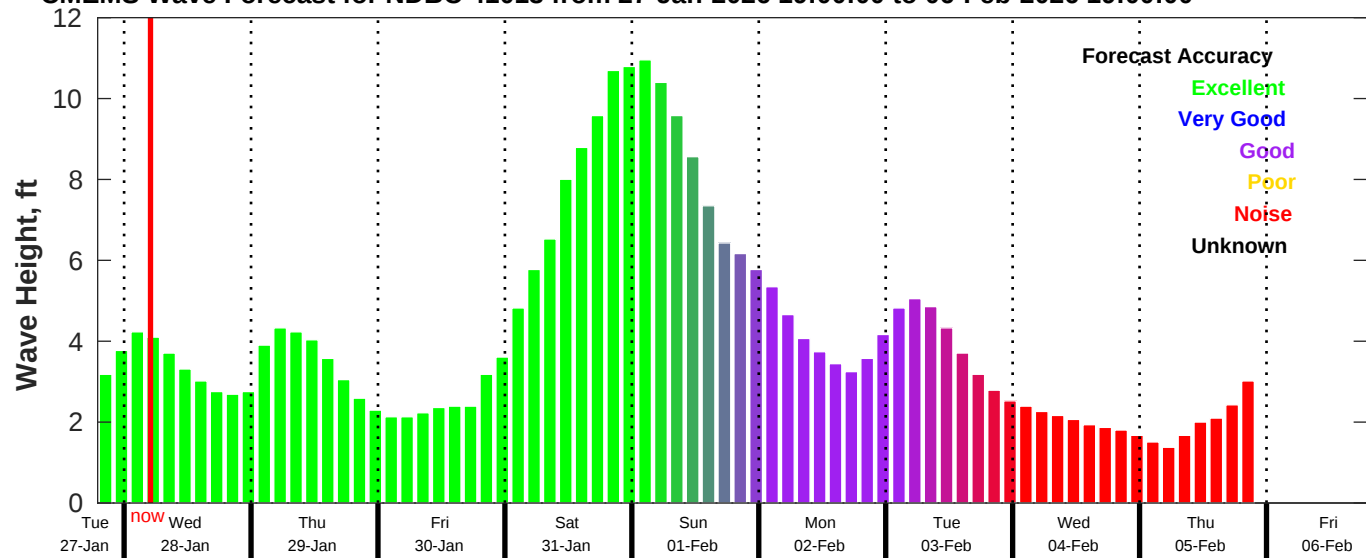
CMEMS Wave Forecast for NDBC 41013 from 27-Jan-2026 19:00:00 to 06-Feb-2026 19:00:00
