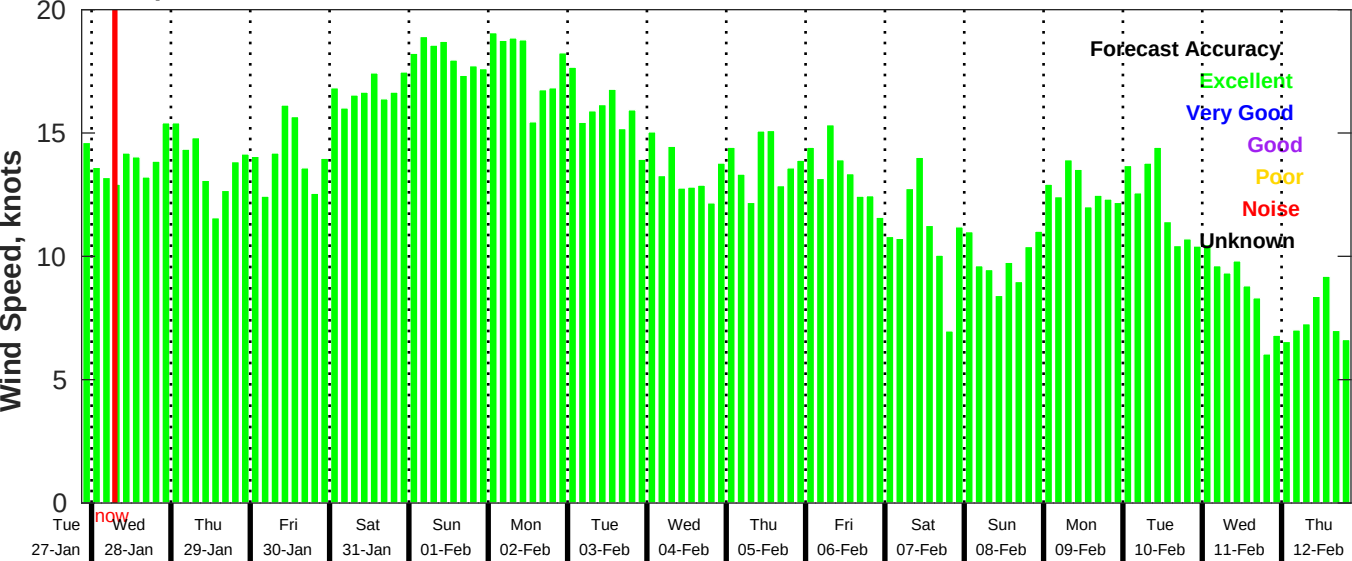
GFS Wind Speed Forecast for NDBC 41040 from 27-Jan-2026 21:00:00 to 12-Feb-2026 21:00:00
